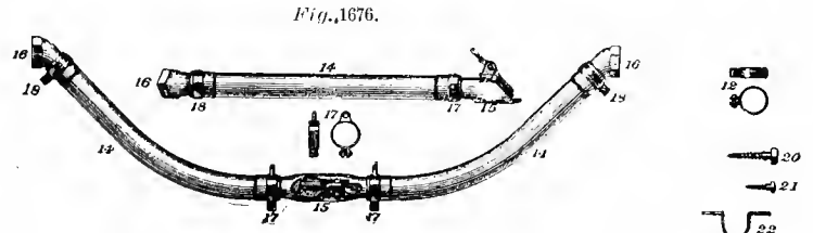
Figs. 1677-1679. EAMES VACUUM BRAKE HOSE.
